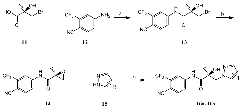
Scheme 1. Synthesis of Pyrazol-1-yl-propanamides 16a–16x a
