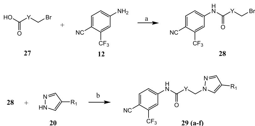
Scheme 4. Synthesis of Pyrazol-1-yl-propanamides 29a–29f a
